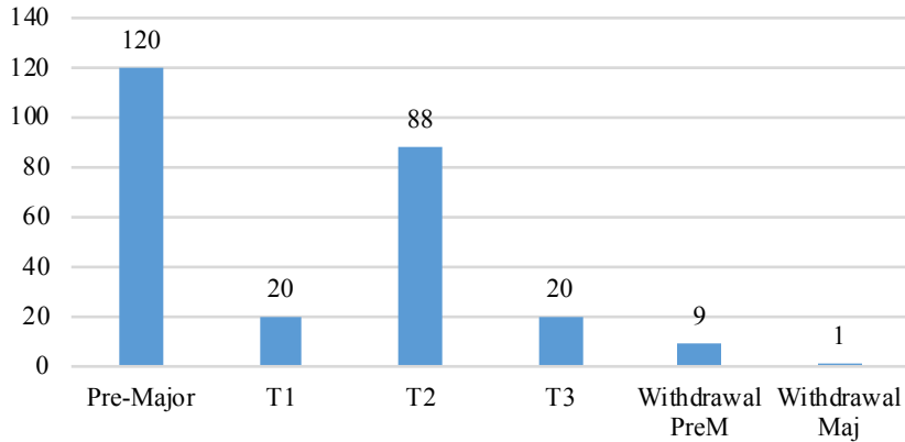
Figure 1. Program Flow
