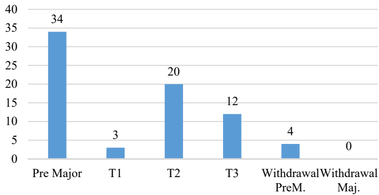
Figure 1. Program Flow
