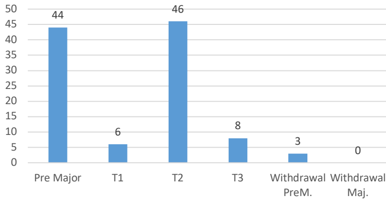
Figure 1. Program Flow
