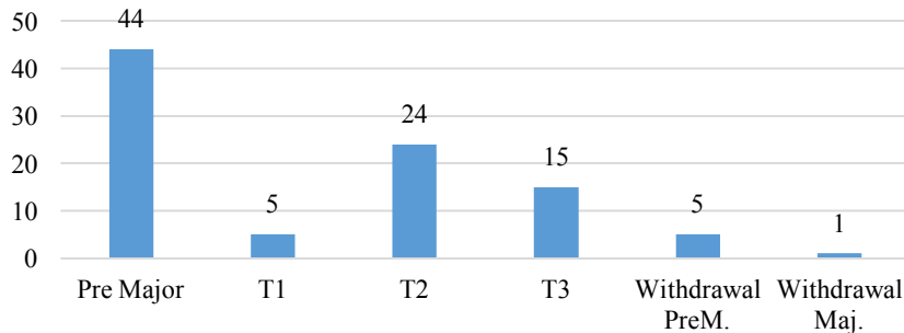
Figure 1. Program Flow
