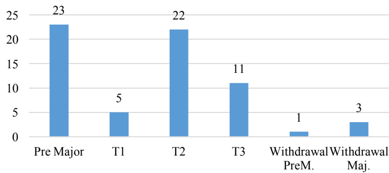
Figure 1. Program Flow
