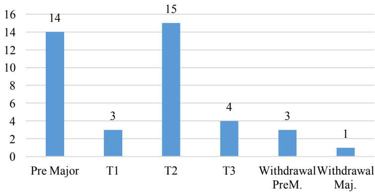
Figure 1. Program Flow
