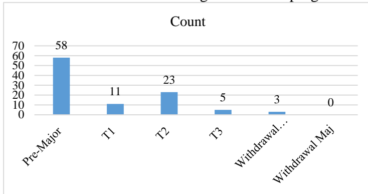
Figure 1. Program Flow
