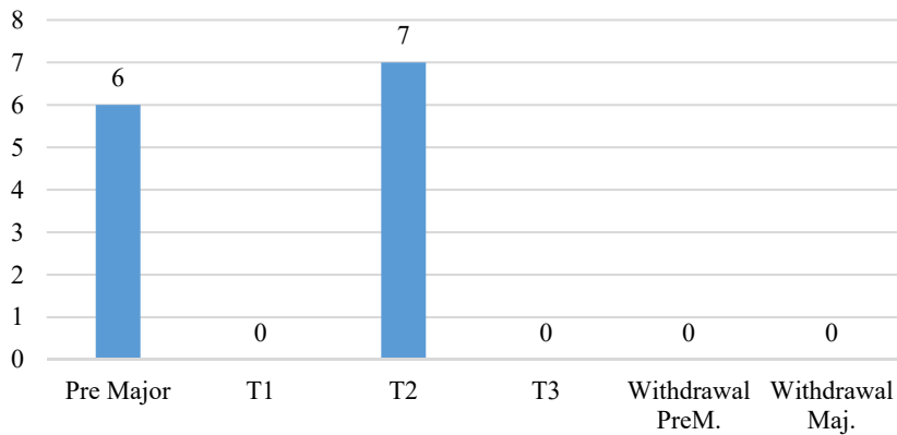
Figure 1. Program Flow
