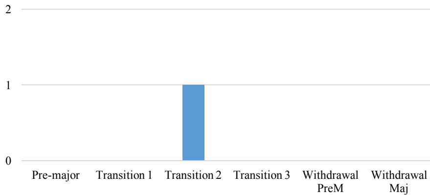
Figure 1. Program Flow
