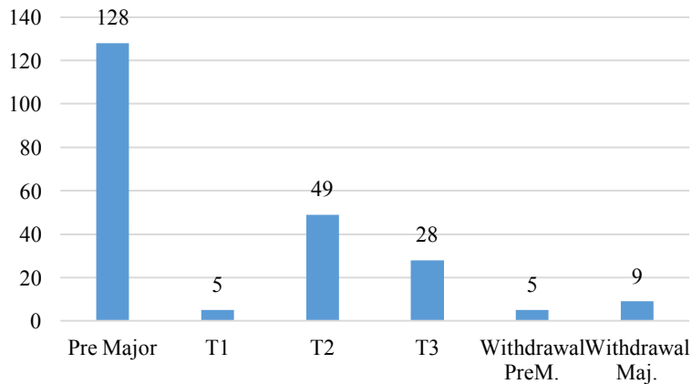
Figure 1. Program Flow
