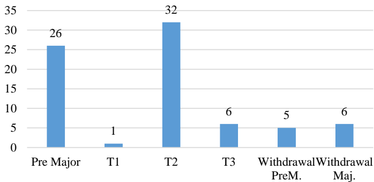
Figure 1. Program Flow
