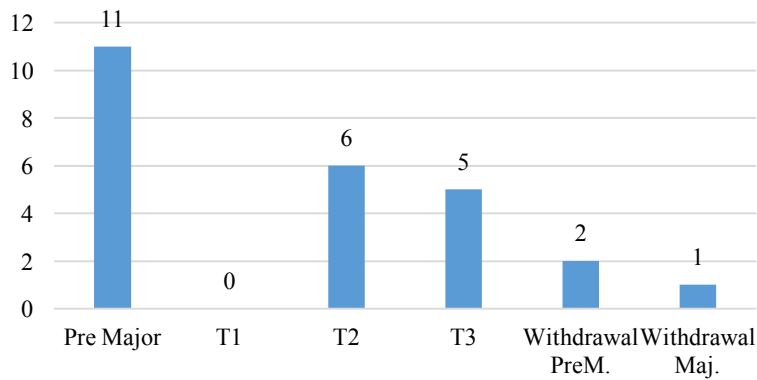
Figure 1. Program Flow
